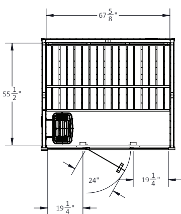
Top Down View w/ Interior Measurements
